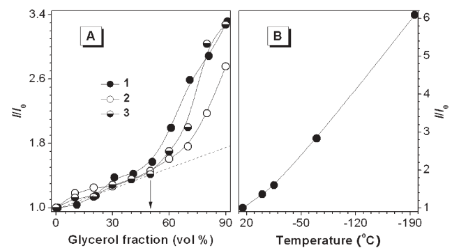
Fig. 2 (A) Changes in the PL peak intensities ( I ) of the solutions of 1–3 (20 \mu\text{M} ) with the glycerol contents in the ethanol/glycerol mixtures. I_0 = intensity in pure ethanol solution. (B) Temperature effect on the PL peak intensity of 3 . I_0 = intensity at room temperature (25 ^{\circ}\text{C} ).
